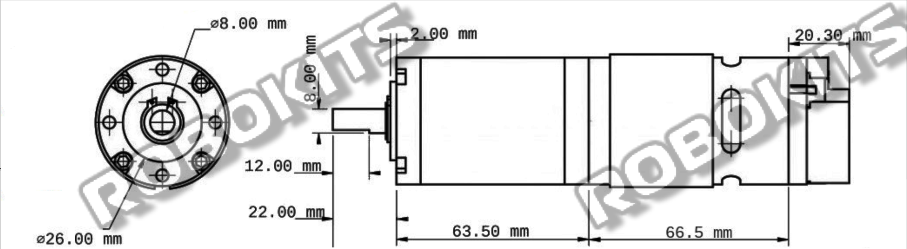
Mechanical Drawing (Dimensions are in mm)
