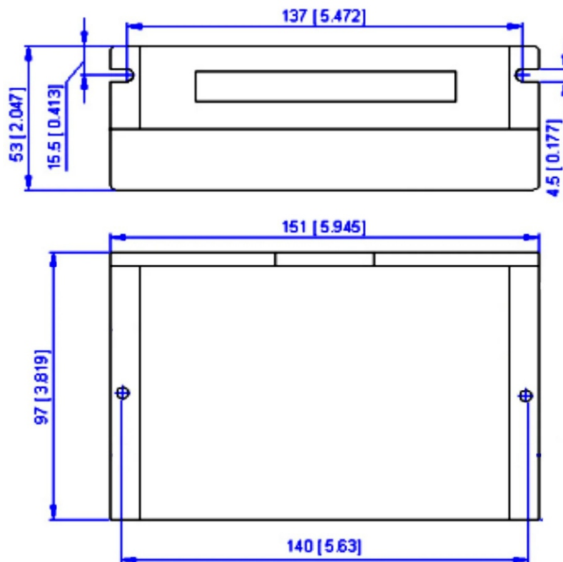
Figure 1: Mechanical specifications
