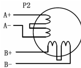
Figure 8: 8-lead motor series connections
