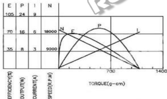
Base Motor Characteristic Graph
